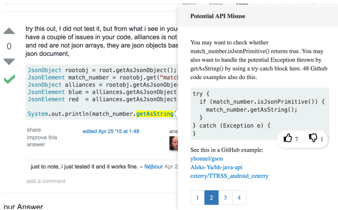
Figure 4: Another API usage warning that reminds programmers to check whether the JsonElement object represents a JSON primitive value by calling the isJsonPrimitive method. It also suggests to catch potential exceptions thrown by getAsString .
