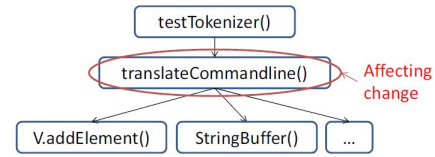
Figure 7. The ECG of testTokenizer
