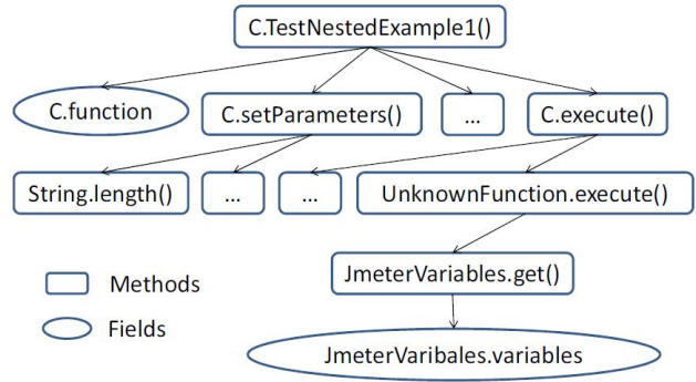
Figure 2. An example extended call graph
