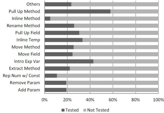
Figure 6. Refactoring test coverage by type
